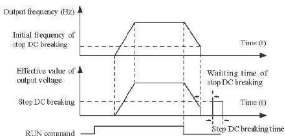
Figure 4-3 Stop DC braking process
